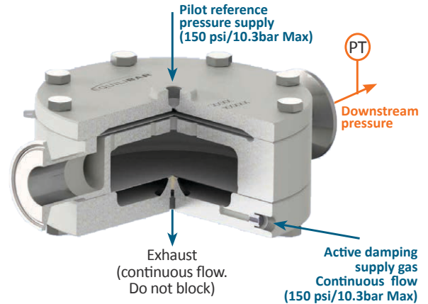
Fig. 2 Cut view of FDO with Active Damping (AD)
